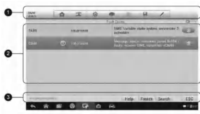
Figure 4-12 Sample Read Codes Screen
